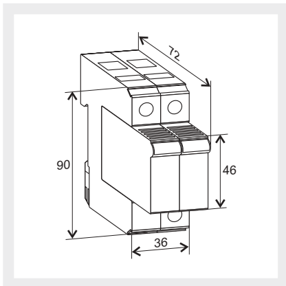
TNS / TNC (2+0) single-phase network
