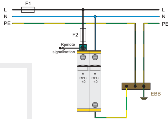
TNS / TNC (2+0) single-phase network
